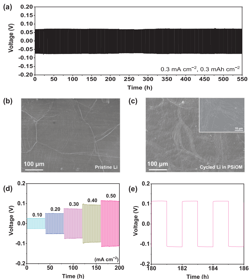
Figure 3. a) Lithium stripping and plating experiment via galvanostatic cycling of Li|PSiOM|Li cells, applying a current density of 0.3 mA cm -2 for 1 h (each step), i.e., cycling a total capacity of 0.3 mAh cm -2 . b,c) SEM micrographs of the b) pristine and c) cycled lithium foil; a magnification of the latter is provided as inset. d) Lithium stripping and plating experiment via galvanostatic cycling of Li|PSiOM|Li cells, applying varying current densities and e) a magnification of representative stripping and plating cycles at 0.5 mA cm -2 .
